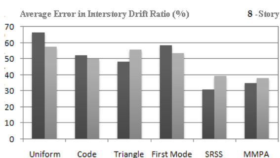
Comparsion Results of NDA and NSPs Method with FEMA-356 and FEMA-440-DM
